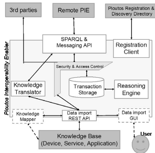
Fig. 3. Functional component diagram of the Plutos Interoperability Enabler (PIE).
