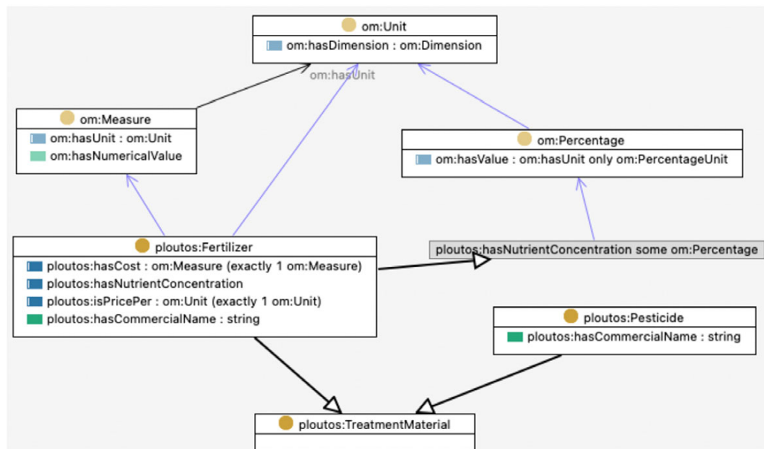
Fig. 8. OWL diagram of the Plutos class TreatmentMaterial containing fertilisers and pesticides and reusing OM classes.
